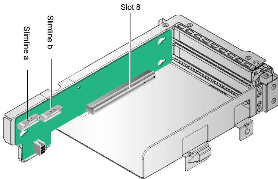
Figure 4-15 Riser card 6 (one x16 slot)
