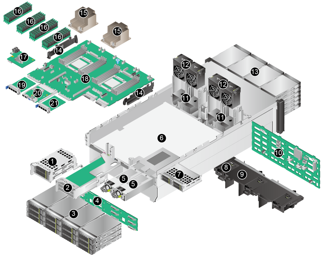
Figure 4-18 Components of the server powered by Kunpeng 920 5220 or 3210 processors
