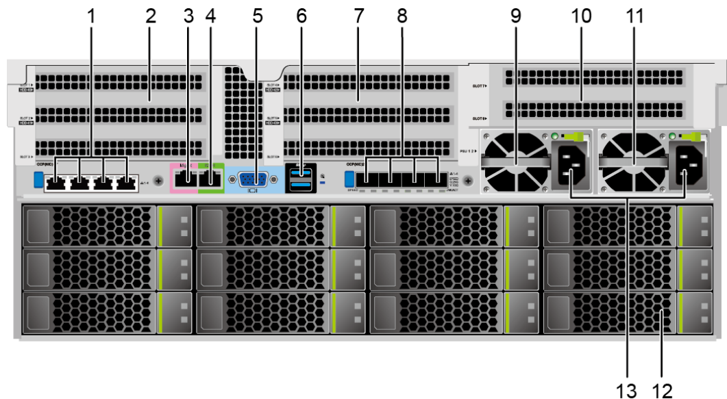
Figure 4-3 Rear Panel Components
