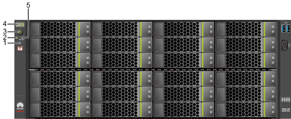
Figure 4-4 Indicators and buttons on the front panel of the server
