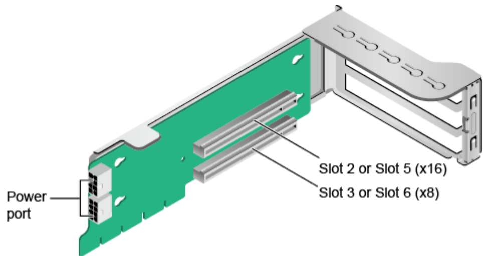
Figure 4-11 Riser card 2 (one x8 slot and one x16 slot)
