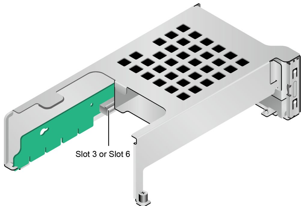
Figure 4-12 Riser card 3 (one x16 slot)
