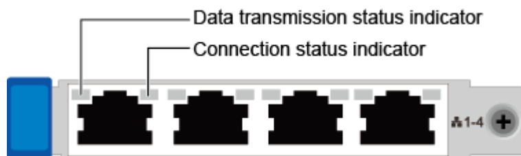
Figure 4-8 TM210 four GE electrical ports
