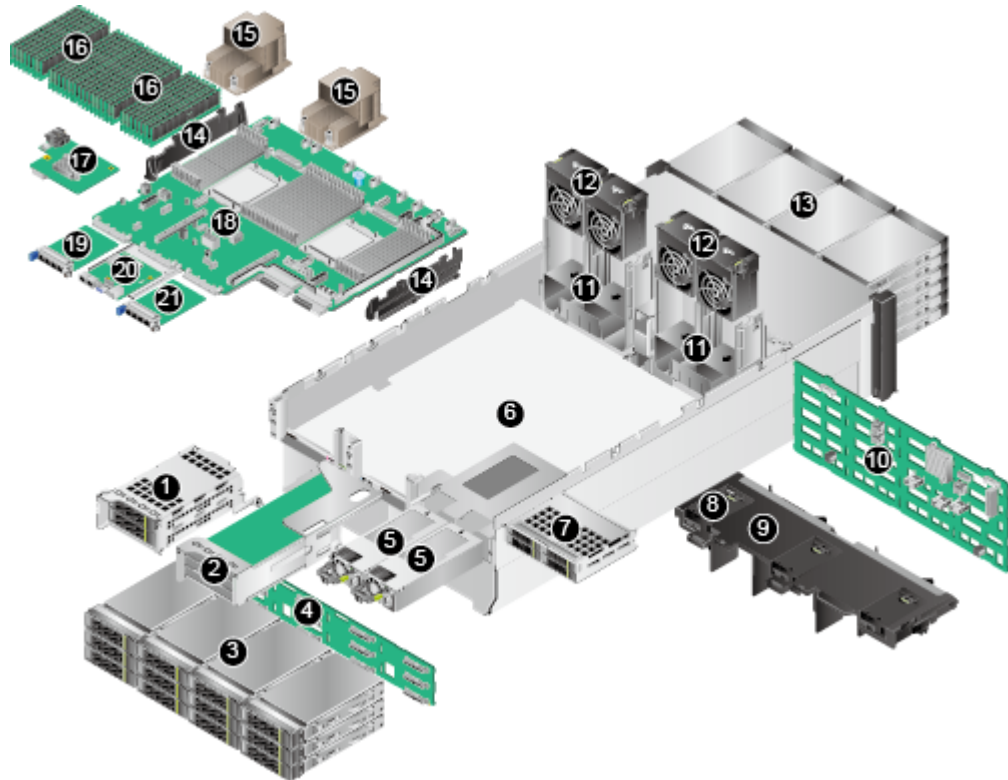
Figure 4-17 Components of the server powered by Kunpeng 920 7260, 5250, 5240, or 5230 processors
