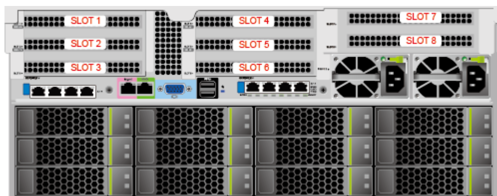
Figure 4-16 PCIe slots
