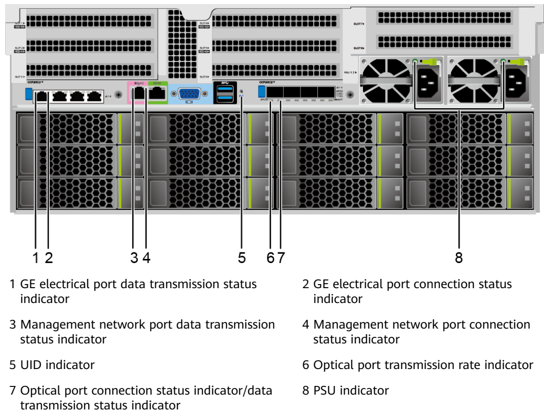
Figure 4-5 Rear panel indicators
