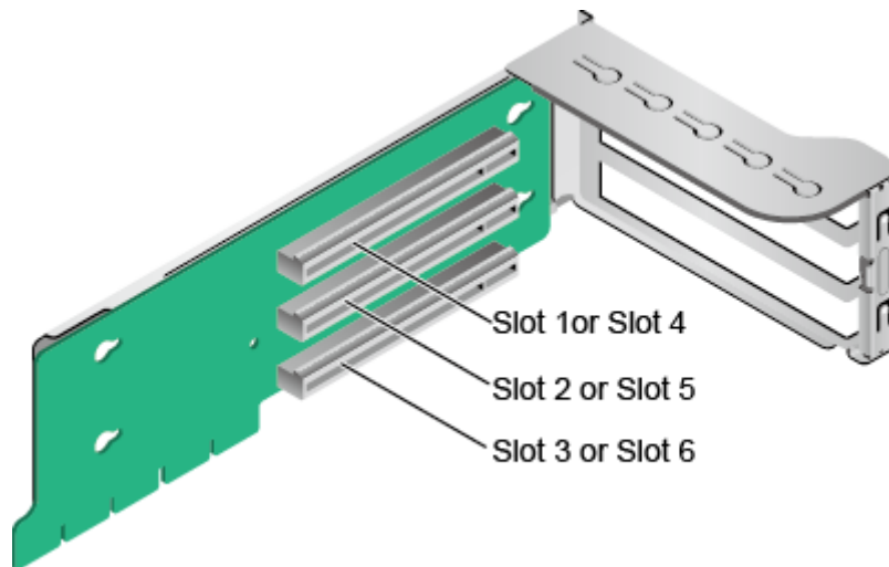
Figure 4-10 Riser card 1 (three x8 slots)
