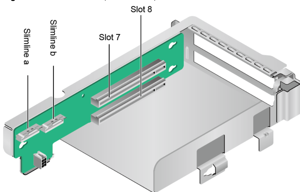
Figure 4-14 Riser card 5 (two x8 slots)
