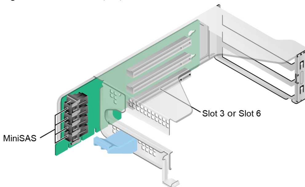
Figure 4-13 Riser card 4 (SAS)
