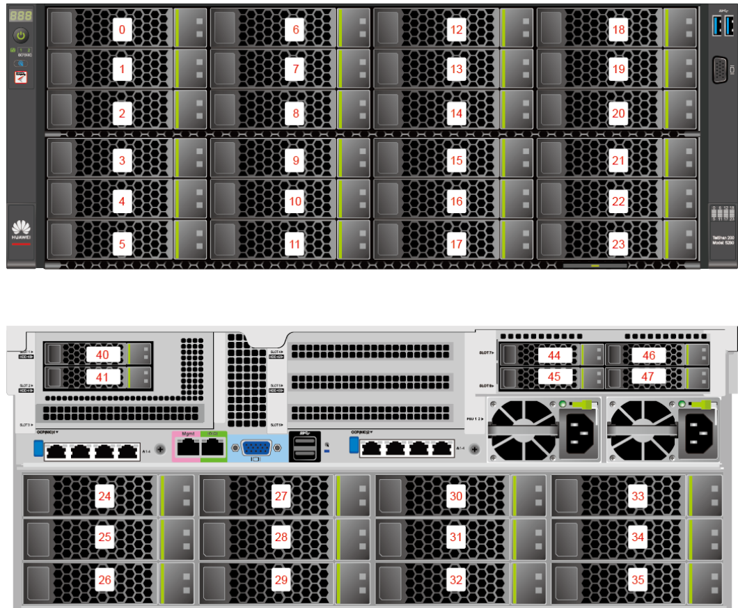
Figure 6-4 Server with 36 x 3.5-inch drives in pass-through mode
